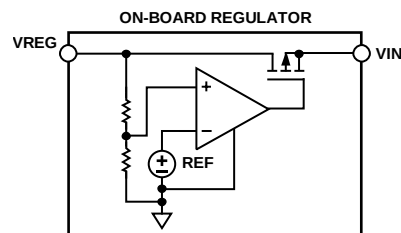
Figure 67. On-Board Regulator
