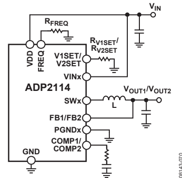
Figure 70. Configuration for Fixed Outputs
