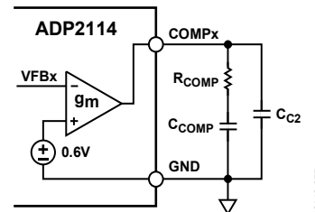
Figure 77. Compensation Components
