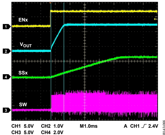
Figure 66. Soft Start
