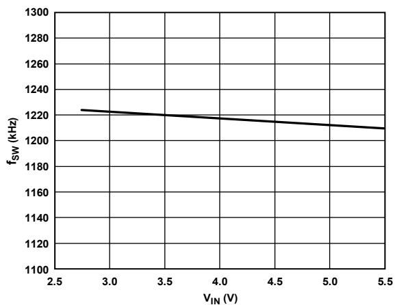
Figure 22. Switching Frequency vs. Input Voltage, f_{SW} = 1.2 MHz
