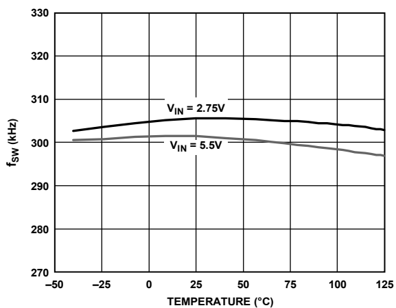
Figure 20. Switching Frequency vs. Temperature, f_{SW} = 300 kHz
