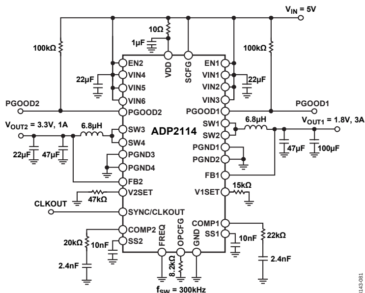
Figure 81. Application Circuit for 3 A/1 A Outputs
