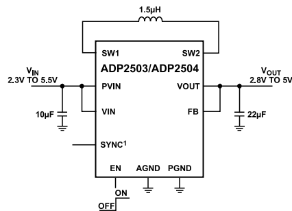
1 ALLOWS THE ADP2503/ADP2504 TO OPERATE IN THREE DIFFERENT MODES.
