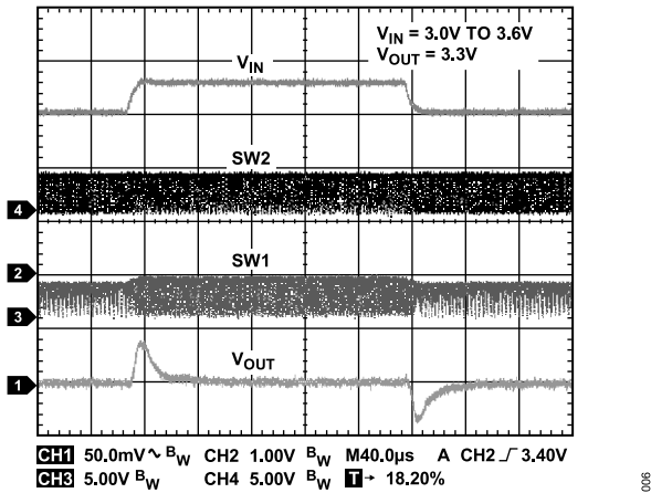
Figure 16. Line Transient, PWM Mode ( V_{IN} = 3.0\text{ V} to 3.6\text{ V} , V_{OUT} = 3.3\text{ V} )
