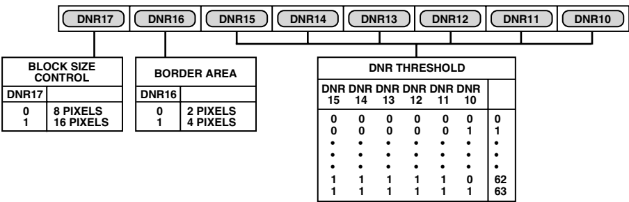
Figure 86. DNR Register 1
