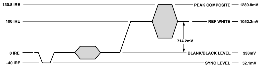
Figure 111. NTSC Composite Video Levels
