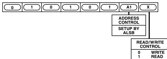
Figure 51. Slave Address
