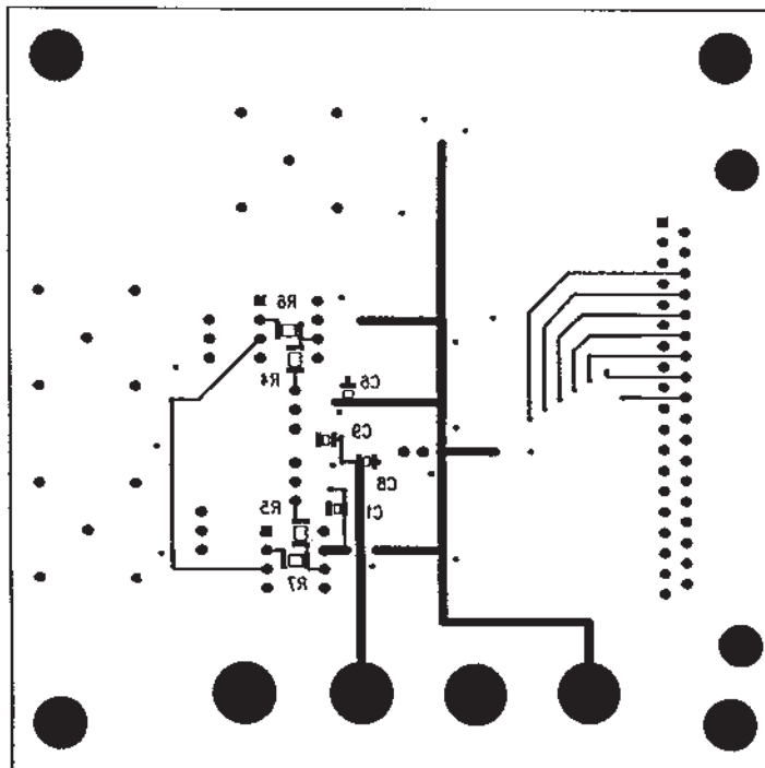
Figure 8. Evaluation Board Layout (Top)
