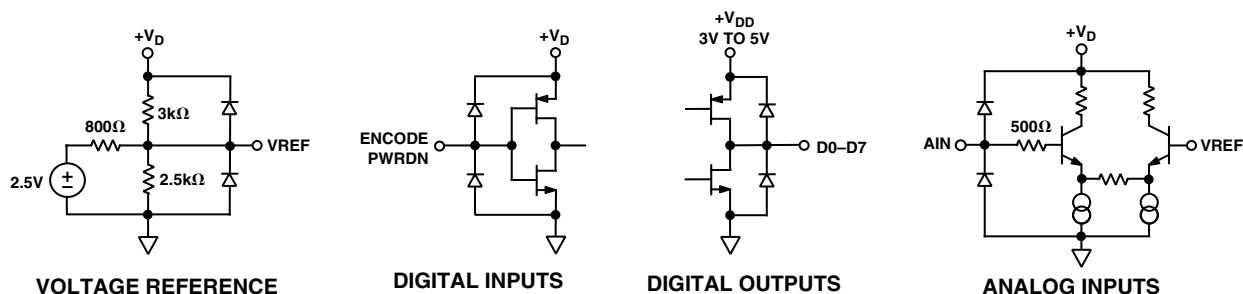
Figure 6. Equivalent Circuits
