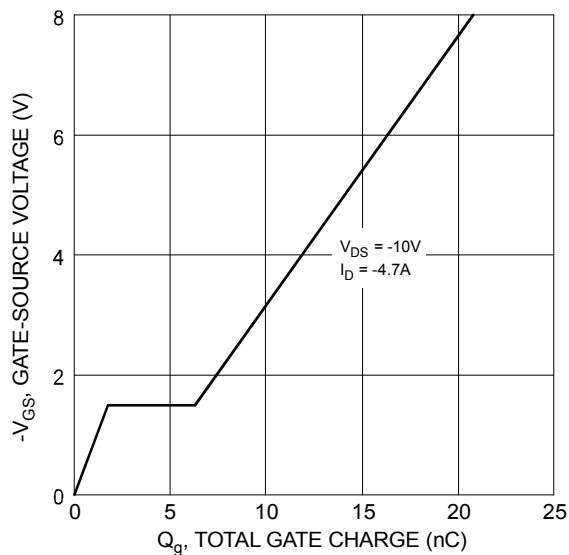
Figure 10 Gate-Charge Characteristics
