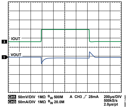
Figure 40. LDO2 Response to Load Transient, IOUT3 from 1 mA to 80 mA, VOUT3 = 3.3 V
