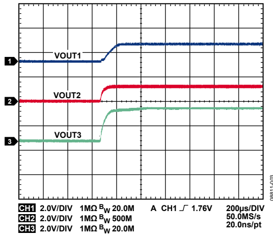
Figure 3. 3-Channel Start-Up Waveforms
