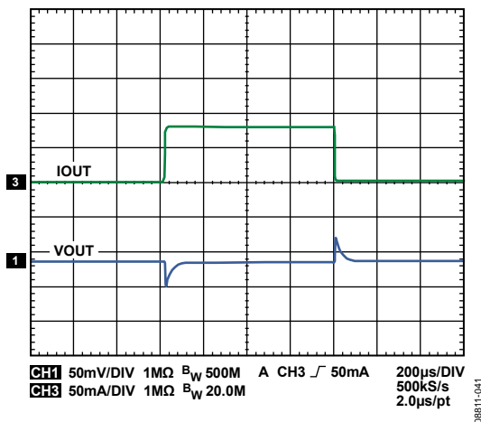
Figure 41. LDO1 Response to Load Transient, IOUT3 from 1 mA to 80 mA, VOUT2 = 1.5 V
