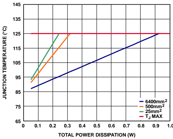
Figure 72. LFCSP, T_A = 85^\circ\text{C}
