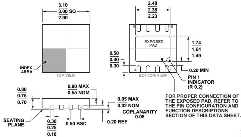
Figure 80. 8-Lead Lead Frame Chip Scale Package [LFCSF_WD] 3 mm x 3 mm Body, Very Very Thin, Dual Lead (CP-8-5) Dimensions shown in millimeters
