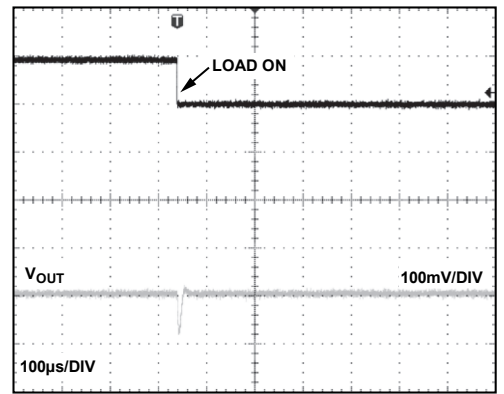
Figure 31. ADR361 Load Transient Response with 0.1 \mu\text{F} Output Capacitor
