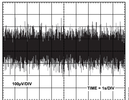
Figure 24. ADR365 10 Hz to 10 kHz Noise
