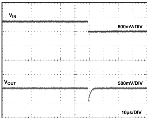
Figure 28. ADR361 Line Transient Response (Decreasing), No Capacitors
