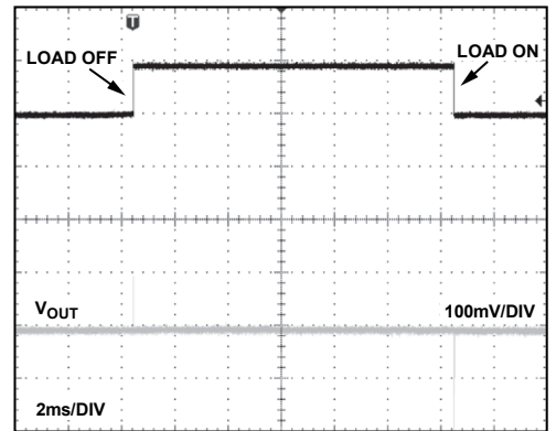
Figure 30. ADR361 Load Transient Response
