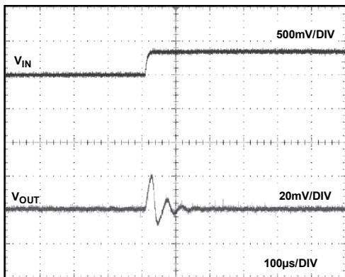
Figure 29. ADR361 Line Transient Response, 0.1 \mu F Input Capacitor
