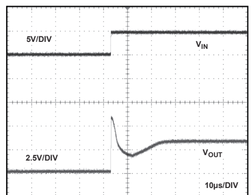
Figure 32. ADR361 Turn On Response Time at 5 V
