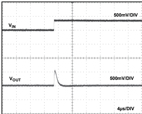
Figure 27. ADR361 Line Transient Response (Increasing), No Capacitors
