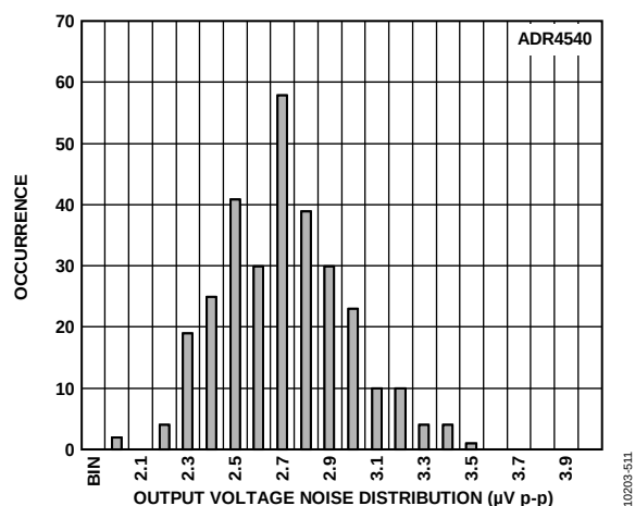
Figure 64. ADR4540 Output Voltage Noise (Maximum Amplitude from 0.1 Hz to 10 Hz)
