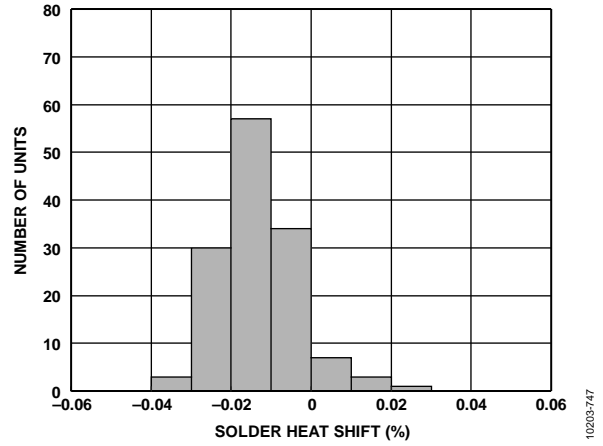
Figure 43. ADR4530 Solder Heat Resistance Shift (3 x Reflow)
