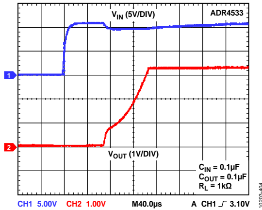
Figure 45. ADR4533 Output Voltage Start-Up Response
