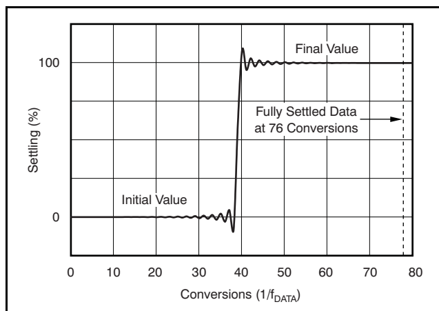
Figure 6. Step Response
