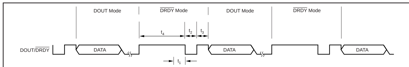
FIGURE 12. DOUT/DRDY Partitioning.
