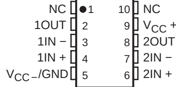
TLV2262M, TLV2262AM U PACKAGE (TOP VIEW)
