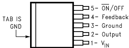
KT Package 5-PIN DDPK/TO-263 Top View
