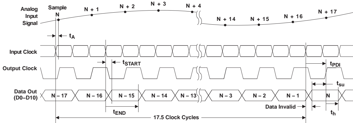
Figure 1. Timing Diagram
