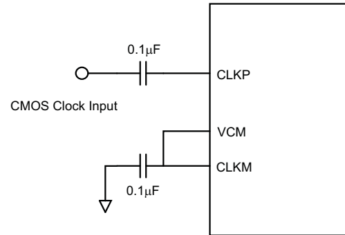
Figure 111. Typical LVCMOS Clock Driving Circuit
