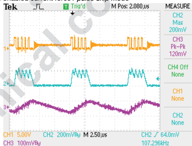
Figure 23. DCDC buck with enabled current force / pulse skip mode
