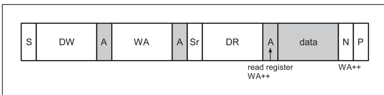
Figure 15. Random Read
