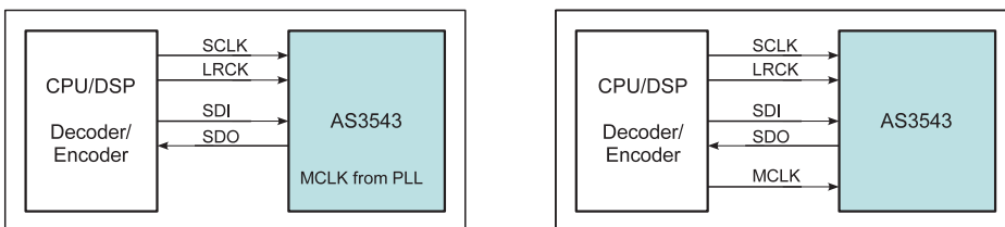
Figure 11. I2S Modes
