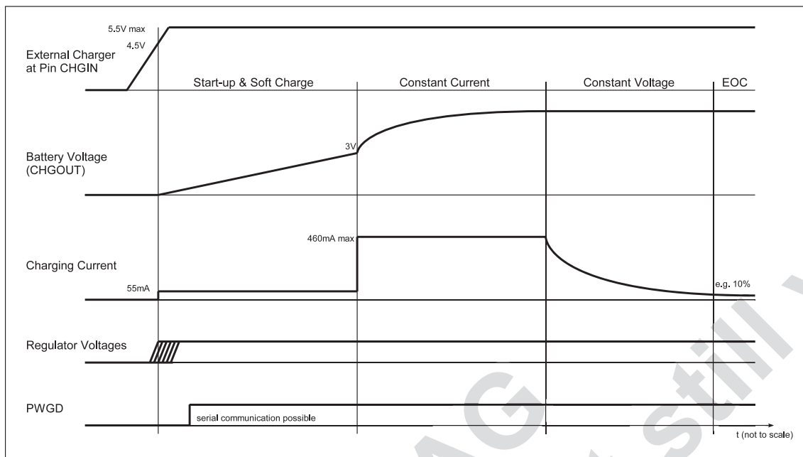
Figure 28. Charger States
