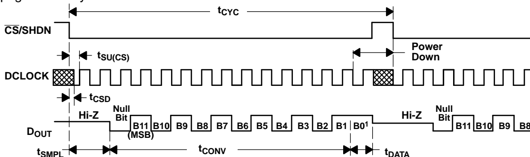
Figure 36. ADS7829 Timing
