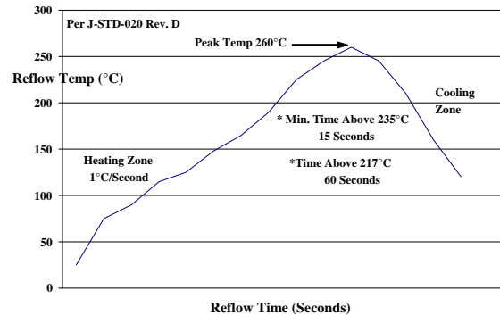
Figure 37. Recommended linear reflow profile using Sn/Ag/Cu solder.
