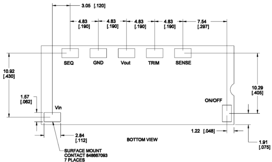
Bottom View
