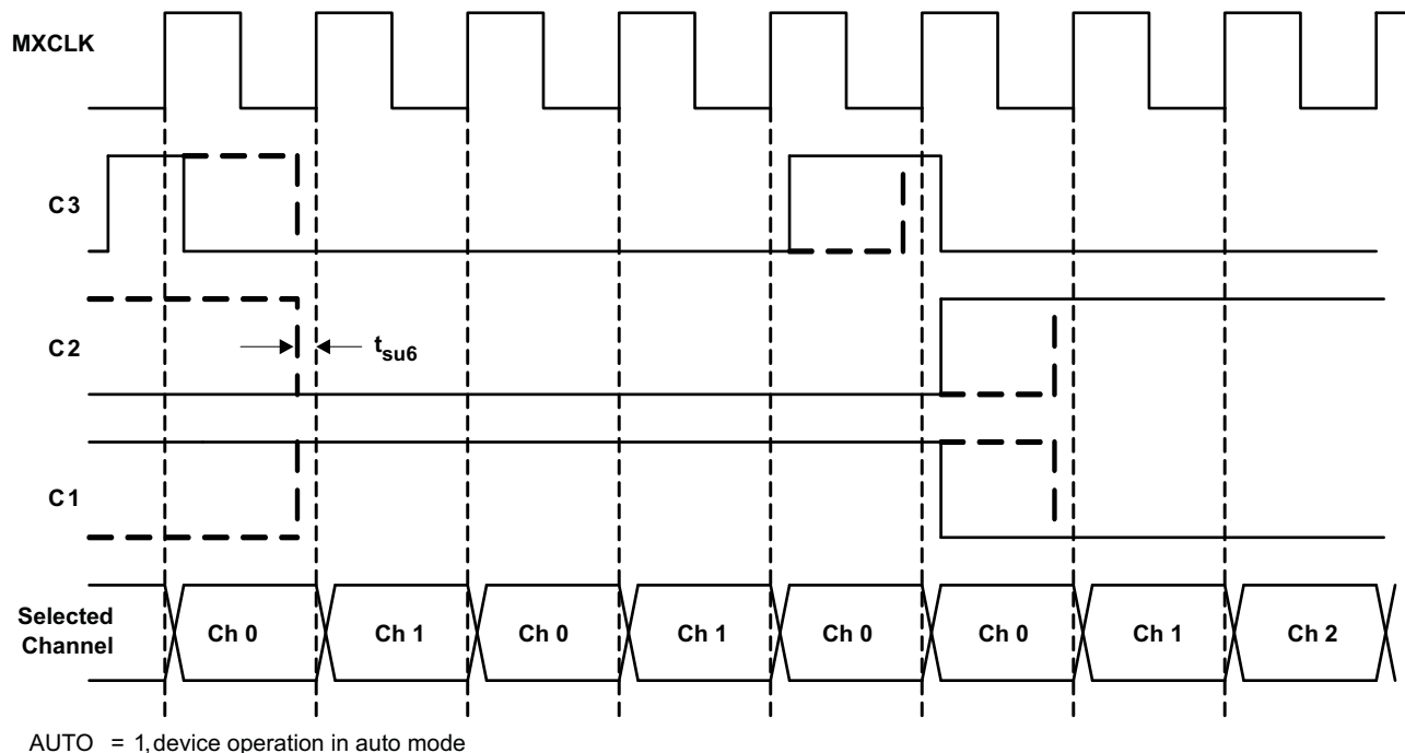
Figure 7. Multiplier Auto Mode Timing Diagram
