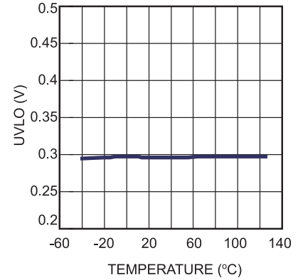
UVLO vs. Temperature
