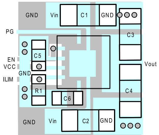
Figure 5: Recommended Layout
