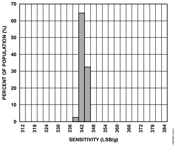
Figure 10. Y-Axis Sensitivity, V_S = V_{DD/IO} = 3.3 V , 25^\circ C
