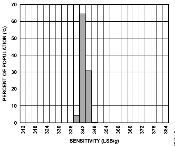
Figure 11. Z-Axis Sensitivity, V_S = V_{DD/IO} = 3.3 V , 25^\circ C
