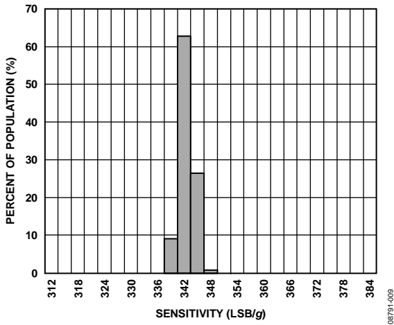
Figure 9. X-Axis Sensitivity, V_S = V_{DD/IO} = 3.3 V , 25^\circ C
