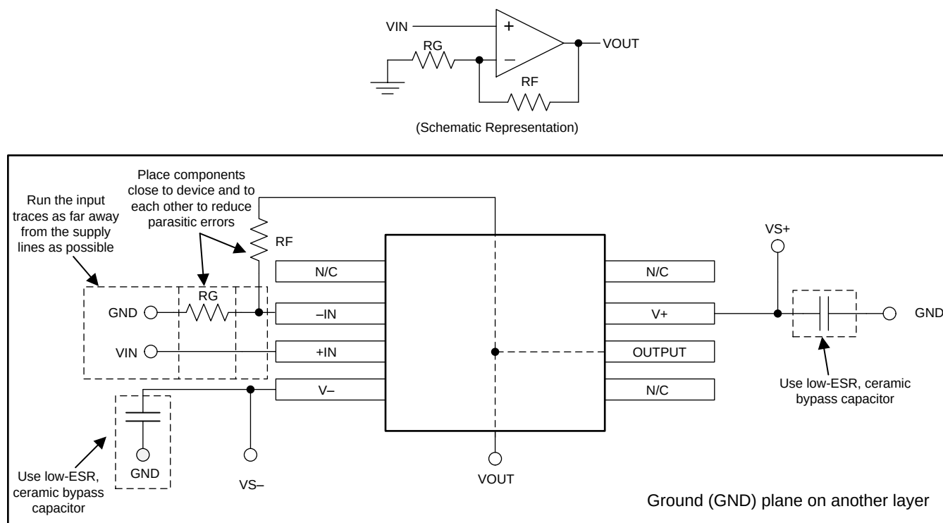
Figure 32. Layout Example
