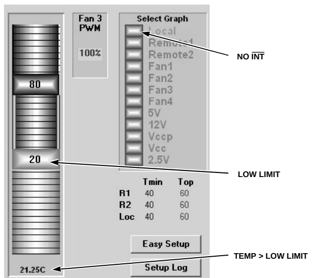
Figure 29. Temperature > Low Limit: No \overline{INT}
