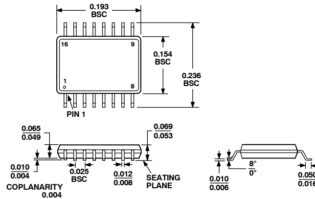
Figure 46. 16-Lead Shrink Small Outline Package [QSOP] (RQ-16)
