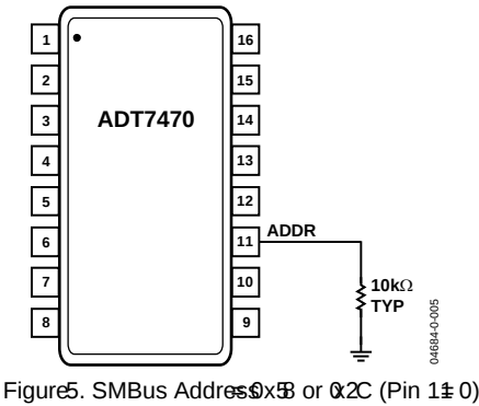
Figure5. SMBus Address = 0x58 or 0x2C (Pin 11 = 0)
