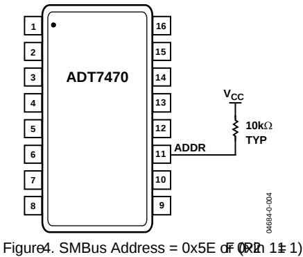
Figure4. SMBus Address = 0x5E (Pin 11 = 1)
