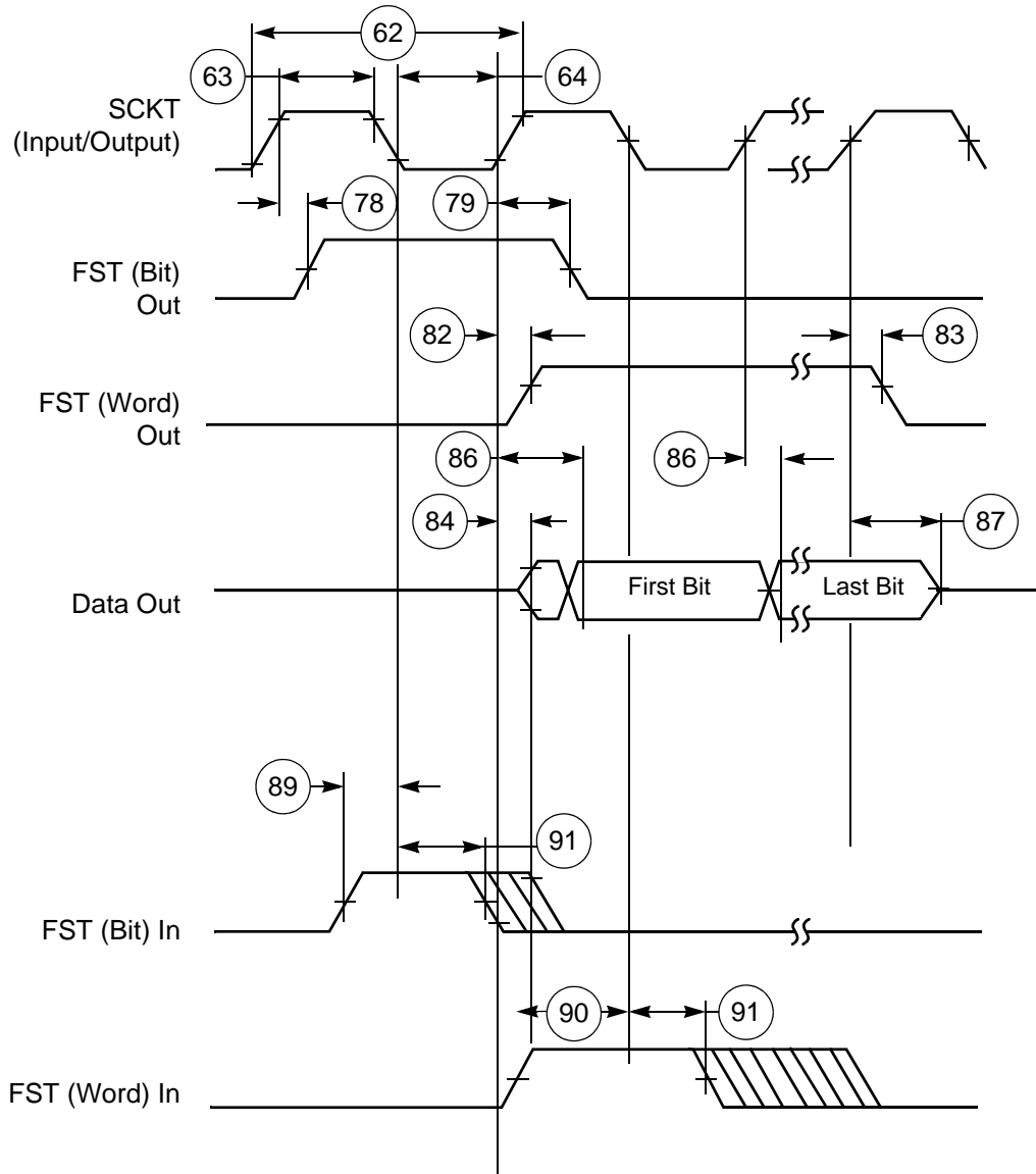
Figure 36. ESAB Transmitter Timing
