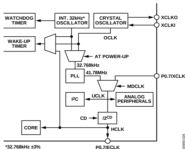
Figure 67. Clocking System
