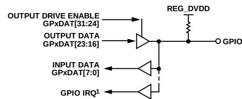
Figure 39. ADuC7033 GPIO
