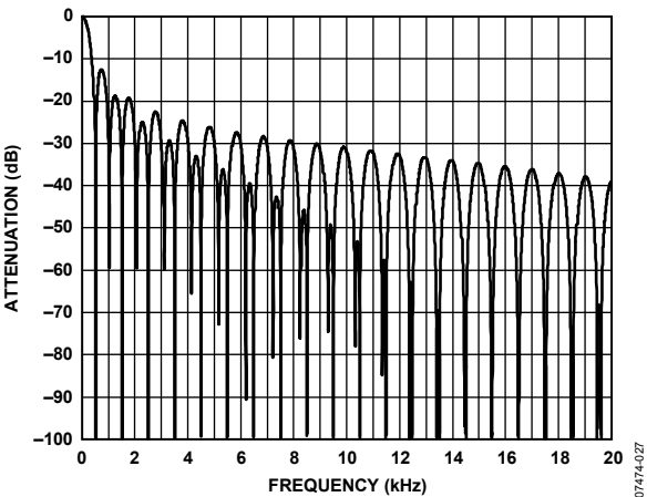
Figure 28. Typical Digital Filter Response at f_{ADC} = 1\text{ Hz} ( ADCFLT = 0xBD1F )
