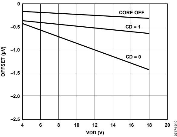
Figure 10. ADC Current Channel Offset vs. V_{DD} @ 25^{\circ}\text{C}
