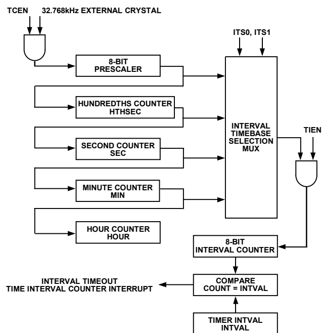
Figure 65. TIC, Simplified Block Diagram
