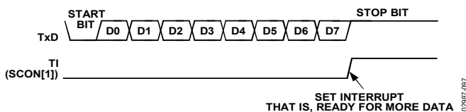
Figure 82. UART Serial Port Transmission, Mode 1
