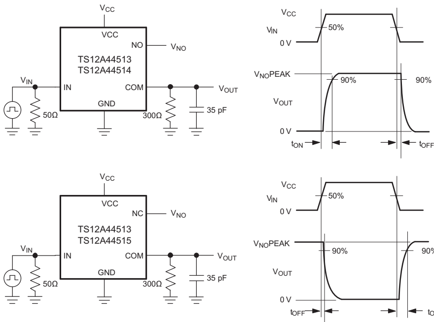
Figure 2. Switching Times
