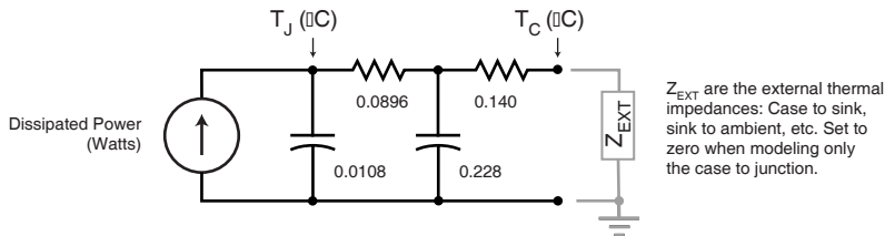
FIGURE 19B, TRANSIENT THERMAL IMPEDANCE MODEL
