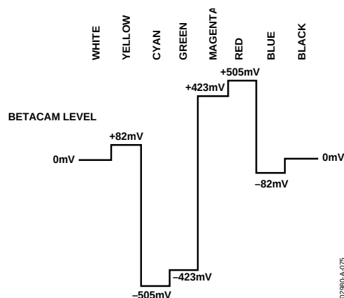
Figure 76. NTSC 100% Color Bars, No Pedestal Pr Levels
