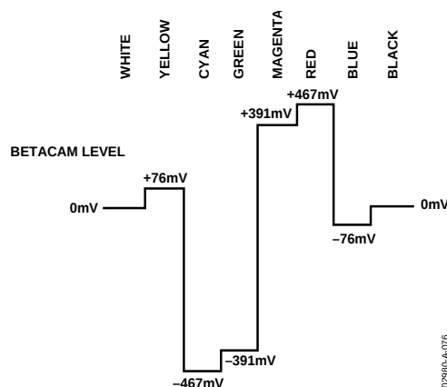
Figure 77. NTSC 100% Color Bars with Pedestal Pr Levels
