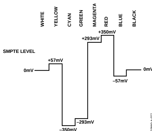
Figure 78. PAL 100% Color Bars, Pr Levels
