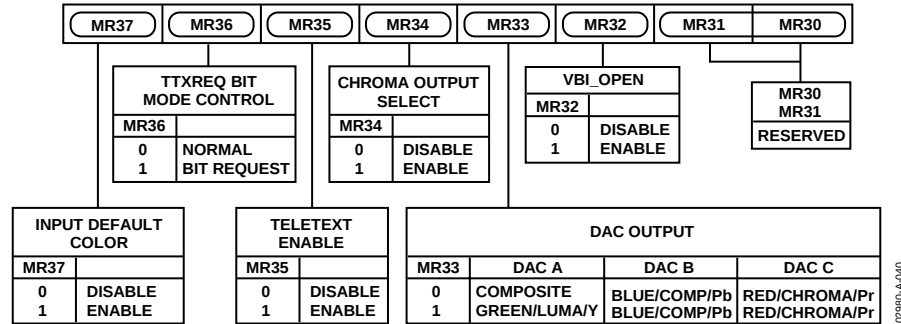
Figure 41. Mode Register 3
