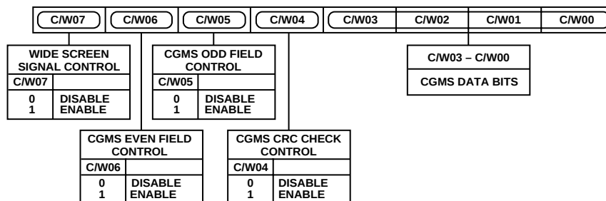
Figure 51. CGMS_WSS Register 0
