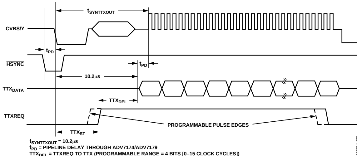
Figure 60. Teletext Functionality
