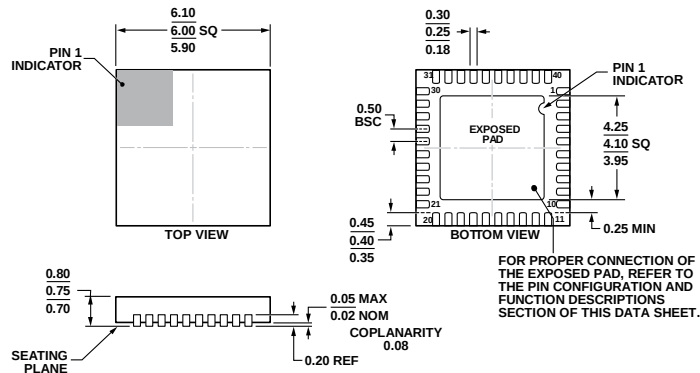
Figure 81. 40-Lead Lead Frame Chip Scale Package [LFCSP_WQ] 6 mm × 6 mm Body, Very, Very Thin Quad (CP-40-9)
