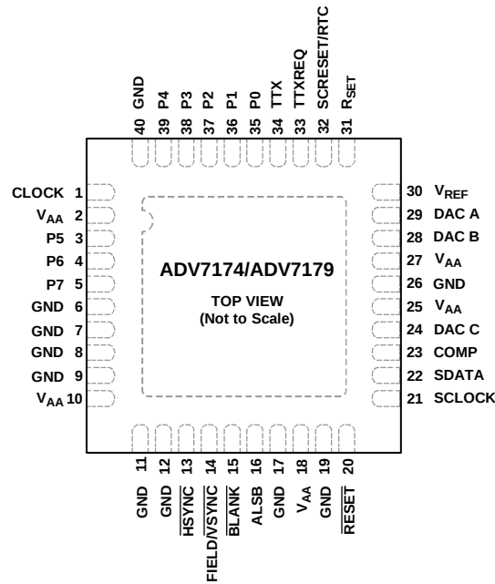
Figure 5. Pin Configurations
