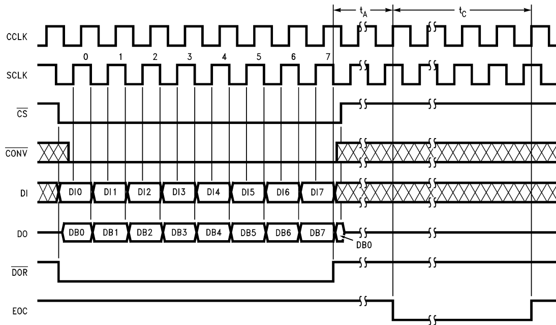
Figure 51. ADC12038 Conversion Using \overline{\text{CS}} with 8-Bit Digital Output Format
