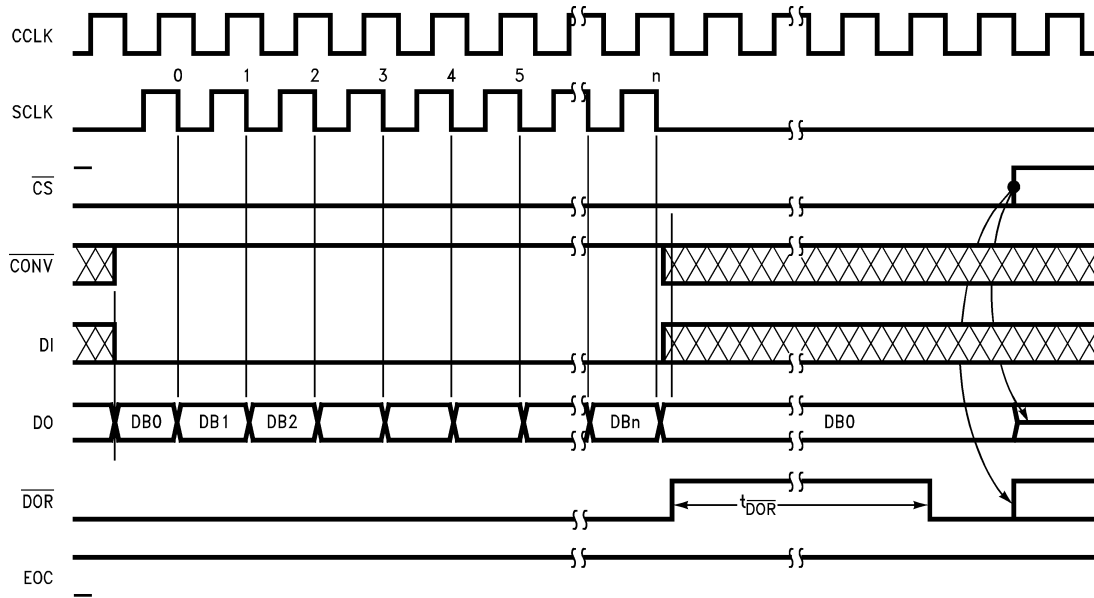
Figure 50. ADC12038 Read Data without Starting a Conversion with \overline{\text{CS}} Continuously Low
