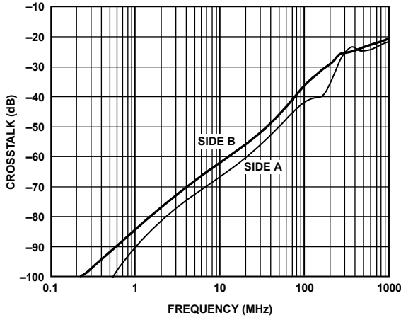
Figure 36. AD8039 Crosstalk, V_{IN} = 1\text{ V p-p} , Gain = +1
