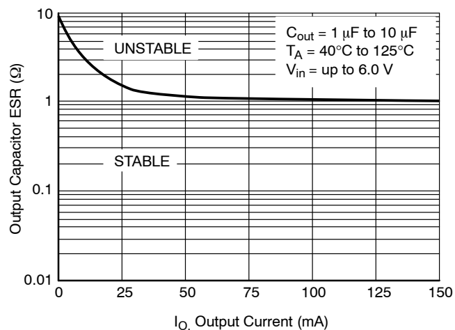
Figure 29. Stability
