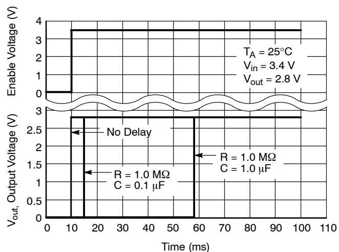
Figure 33. Delayed Turn-on
