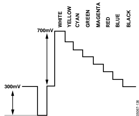
Figure 136. Y Levels—PAL
