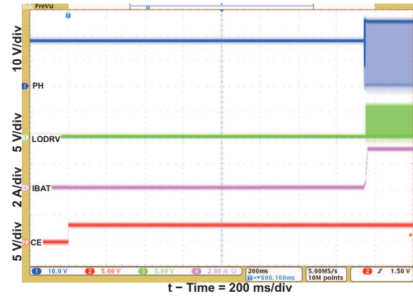
Figure 2. Charge Enable
