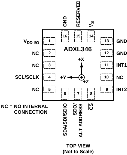
Figure 3. Pin Configuration (Top View)
