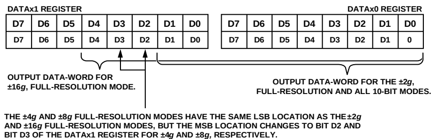
Figure 52. Data Formatting When Output Data Is Right Justified
