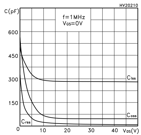
Figure 12. Capacitance variations
