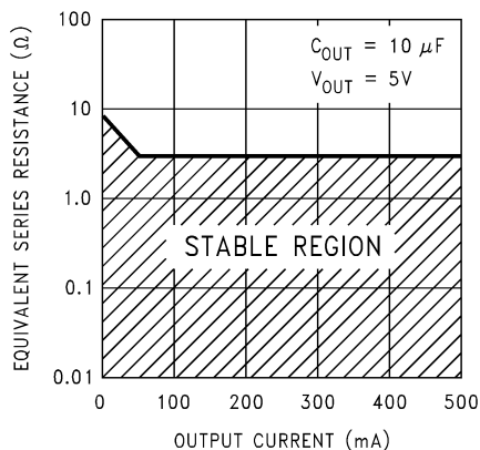
Figure 24. ESR Limits
