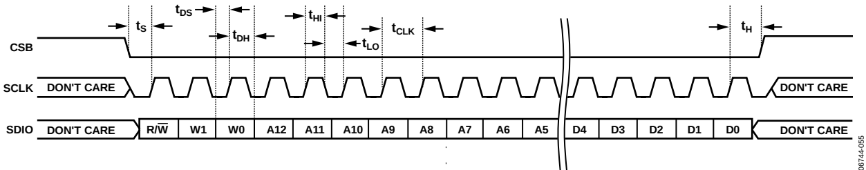
Figure 55. Serial Control Port Write—MSB First, 16-Bit Instruction, Timing Measurements
