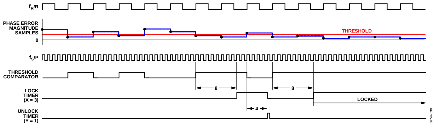
Figure 31. Lock/Unlock Detection Timing
