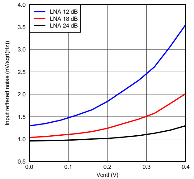
Figure 21. IRN, PGA = 24dB and Medium Power Mode
