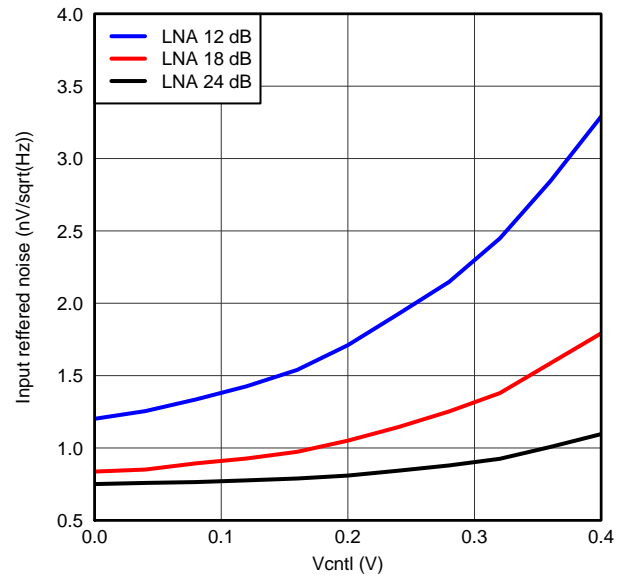
Figure 19. IRN, PGA = 24dB and Low Noise Mode
