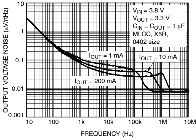
Figure 6. Output Voltage Noise Spectral Density for V_{\text{OUT}} = 3.3\text{ V} , C_{\text{OUT}} = 1\text{ }\mu\text{F}
