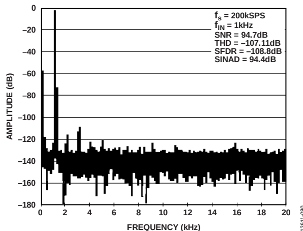
Figure 81. FFT for Driving a Single-Ended to Differential Converter Using Dynamic Power Scaling, -0.5 dBFS, On Time of 4 \mu\text{s} , for the Schematic Shown in Figure 76
