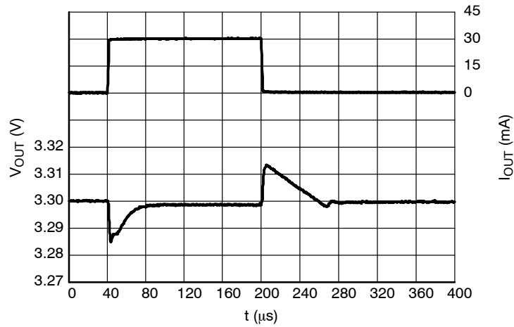
Figure 60. Load Transients, 3.3 V Version, I_{OUT} = 1 - 30 \text{ mA} , t_R = t_F = 0.5 \mu s , V_{IN} = 6.3 V , ECO = H
