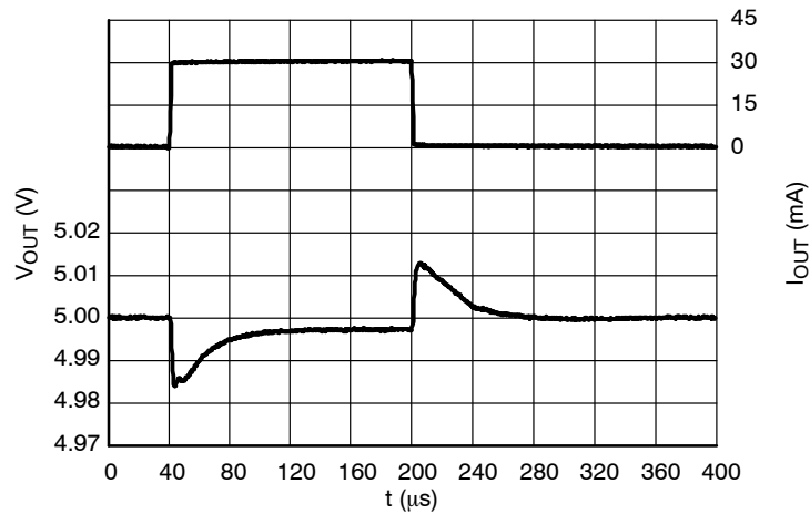
Figure 62. Load Transients, 5.0 V Version, I_{OUT} = 1 - 30 \text{ mA} , t_R = t_F = 0.5 \mu s , V_{IN} = 8.0 V , ECO = H
