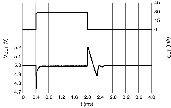
Figure 61. Load Transients, 5.0 V Version, I_{OUT} = 1 - 30 \text{ mA} , t_R = t_F = 0.5 \mu s , V_{IN} = 8.0 V , ECO = L
