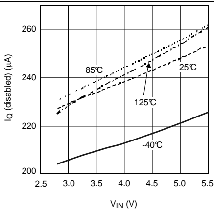
Figure 11. I_Q (disabled) vs V_{IN} and Temperature, EN = 0\text{ V}
